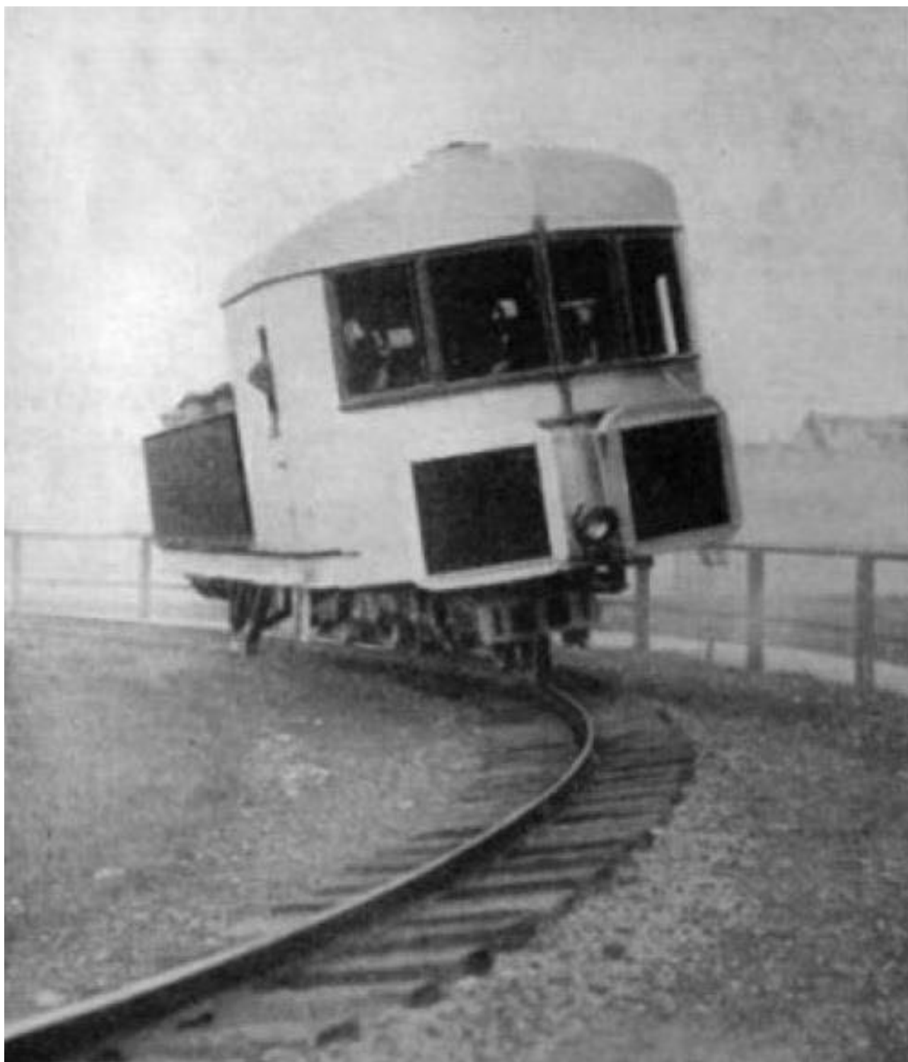
Monorotaia Brennan
